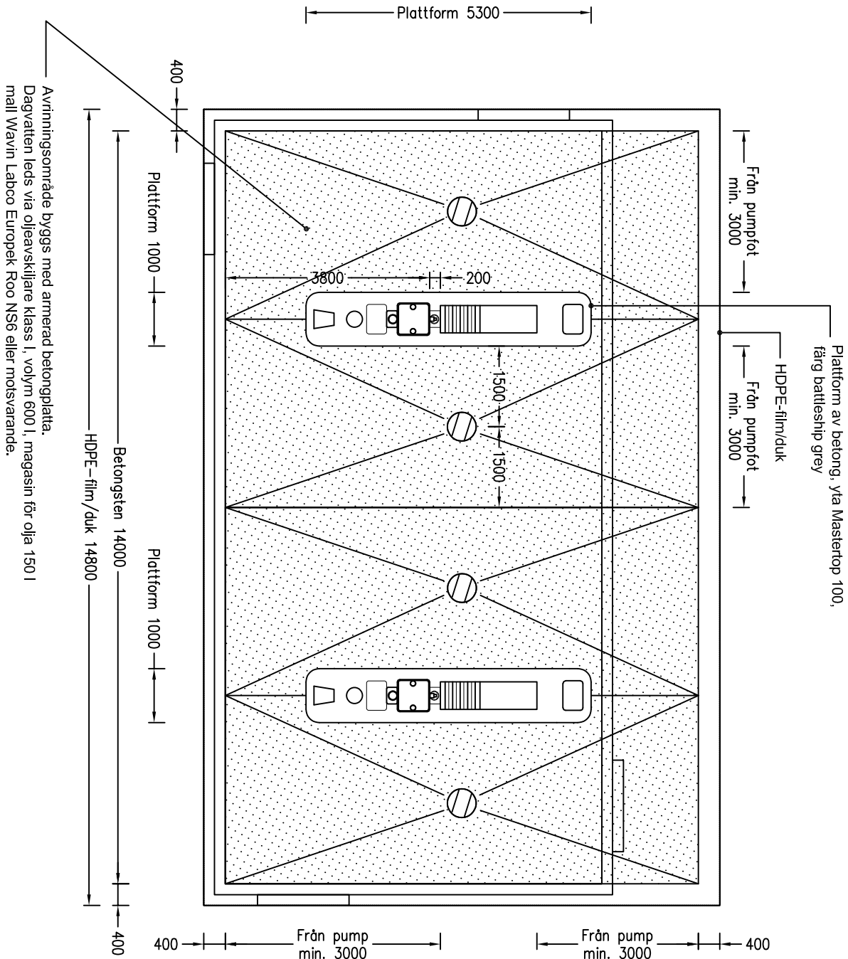
PLANRITNING BENSINSTATION 1:100
